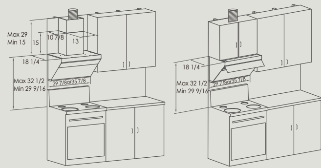
▲ Without upper cabinet+decorative cover ▲ With upper cabinet
