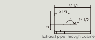
Hole Size of Cabinet on Top Surface
