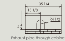
Hole Size of Cabinet on Top Surface
